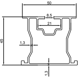
Top Rail YB-M02 872 gr/m
