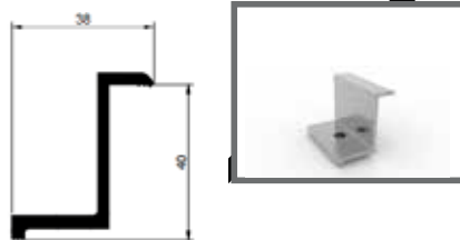
40'lik End Clamp 1621 661 gr/m
