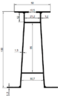
10 cm Profile 100-1 1143 gr/m
