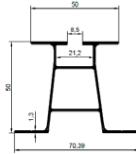
8 cm Profile 80-1 997 gr/m
