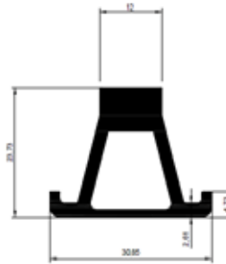
Aluminium Special Nut
