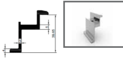
40'lik End Clamps 705 832 gr/m
