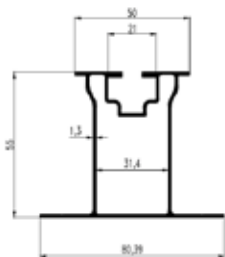
5,5 cm Large Surface Profile 1788 998 gr/m
