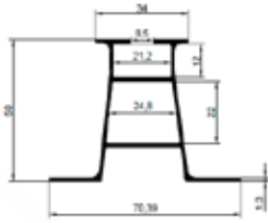
5 cm Small Surface Profile 50-3 737 gr/m
